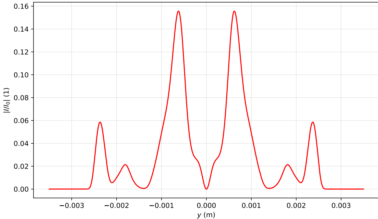
Intensity profile I(x=0, y, z=3.742)/I_0 , P_{in}=9.0P_{cr} , artificial time
